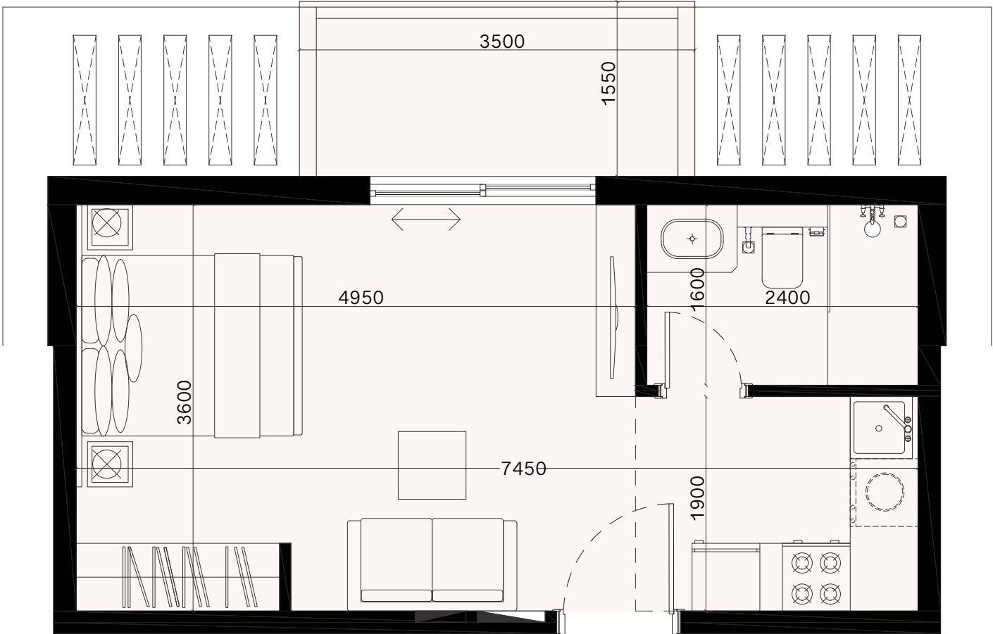
1 ST Floor
